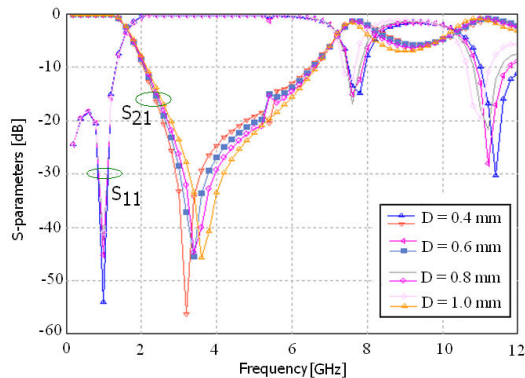
Fig. 6 Magnitudes of the transfer function ( S_{21} ) and input reflection coefficient ( S_{11} ) of the US-DGS LPF for different D
