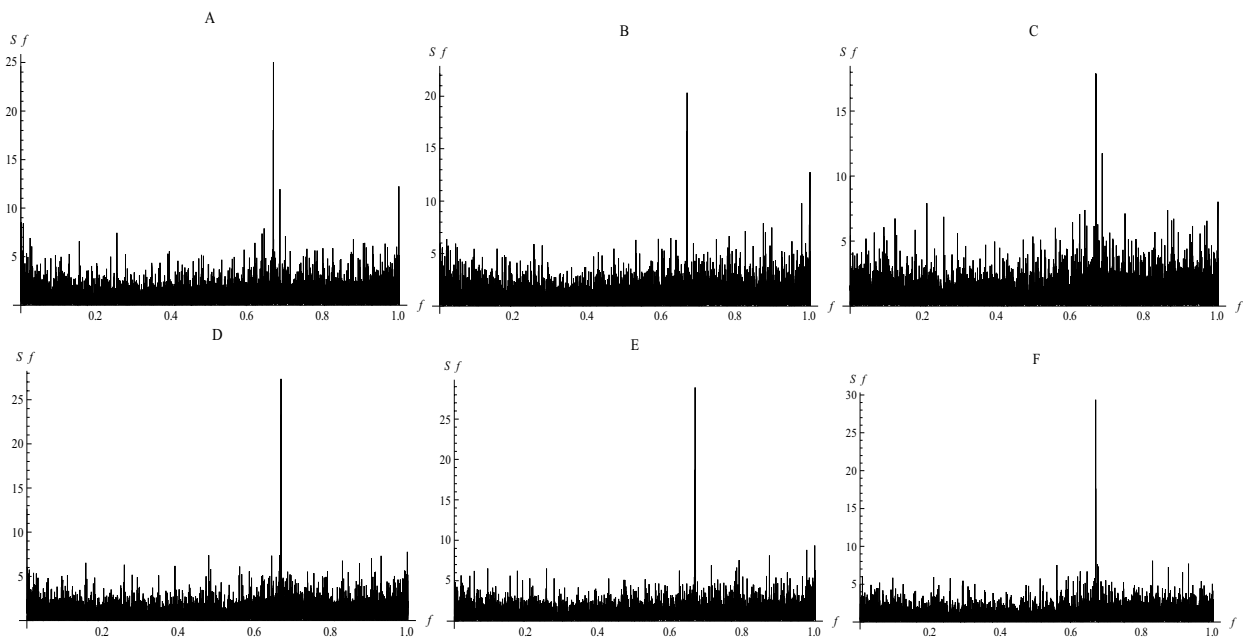
Fig. 3 Power spectra of three aligned HIV-1 whole genomes. A, B and C: the power spectra corresponding to the HIV-1 whole genomes sequences with GenBank accession numbers K03455.1 (HXB2), AB023804.1 and U51188.1, respectively. D, E and F: the power spectra corresponding to the same HIV-1 genomes taken from the base position 700 to 9580.
