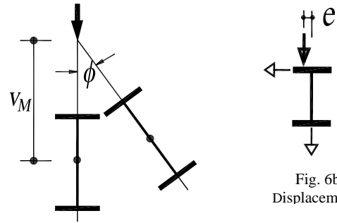
Fig. 6a Section Rotation
