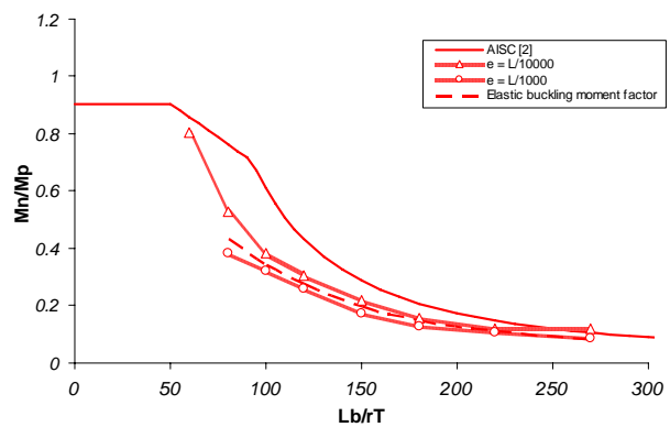
Fig. 11 Flexural Resistance of Type C section
