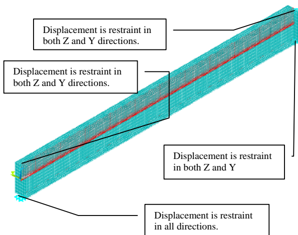
Fig. 2 Model restraints
