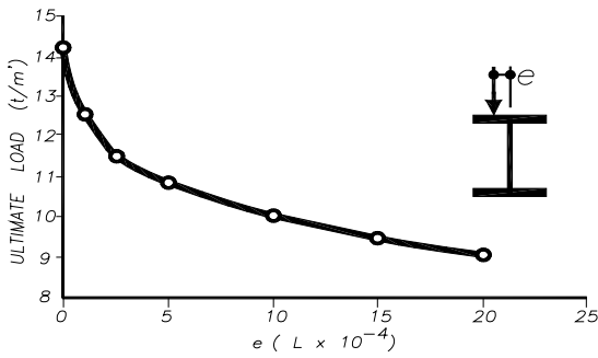
Fig. 8 Imperfection sensitivity
