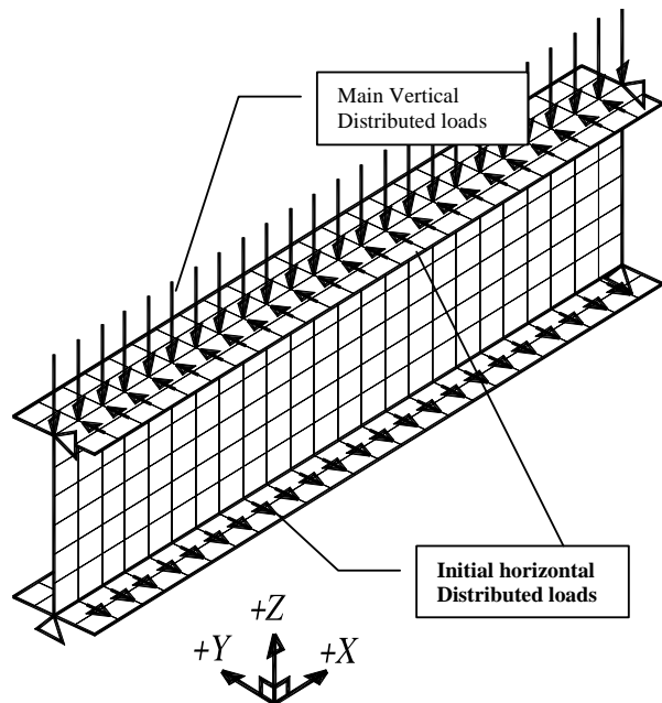
Fig. 3 Loading System
