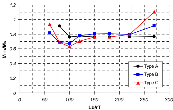
Fig. 13a M_{FE}/M_n – Ratios for e=L/10000 FEA Results
