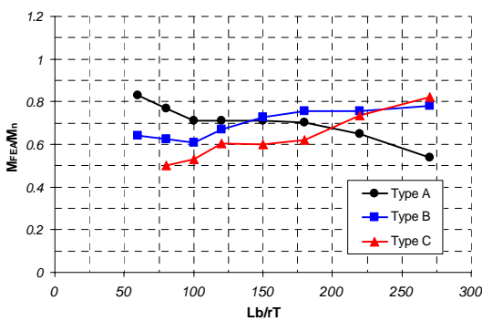
Fig. 13b M_{FE}/M_n – Ratios for e=L/1000
