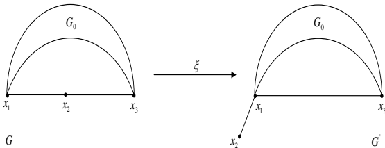
Fig. 1. Transformation C
