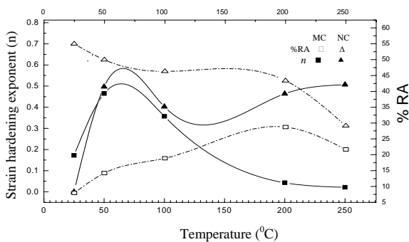
Fig. 4 Variation of strain hardening exponent and the %RA at various test temperatures for MC and NC sample
