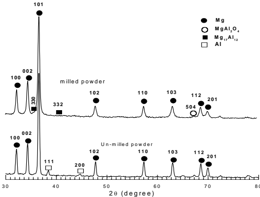
Fig. 1 (a) XRD spectra of milled and unmilled powders
