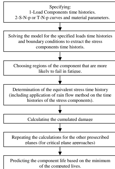
Fig. 4 The proposed numerical life assessment scheme
