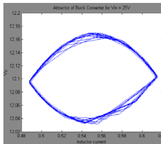
Fig. 4 Period-1 Attractor
