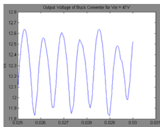
Fig. 7 Chaotic Waveform
