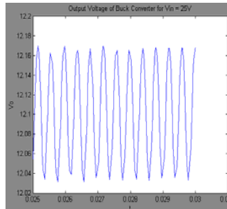
Fig. 3 Period-1 Waveform
