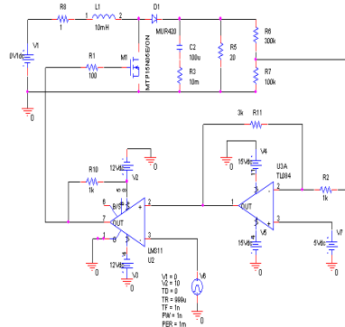
Fig. 2 PWM boost converter
