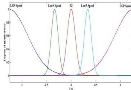
Fig. 5 Linear velocity in x-direction membership function
