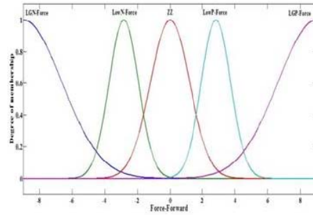
Fig. 4 Forward force membership function
