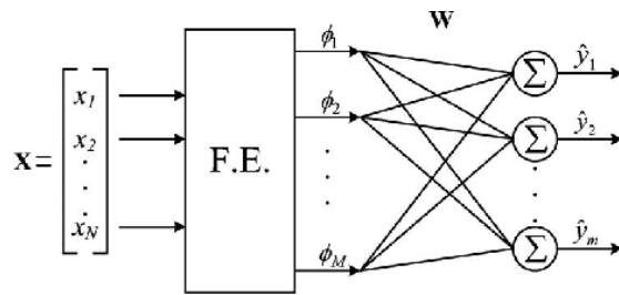
Fig. 7 FLNN structure
