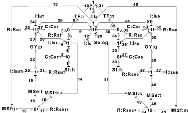
Fig. 7. BGI of an active suspension.
