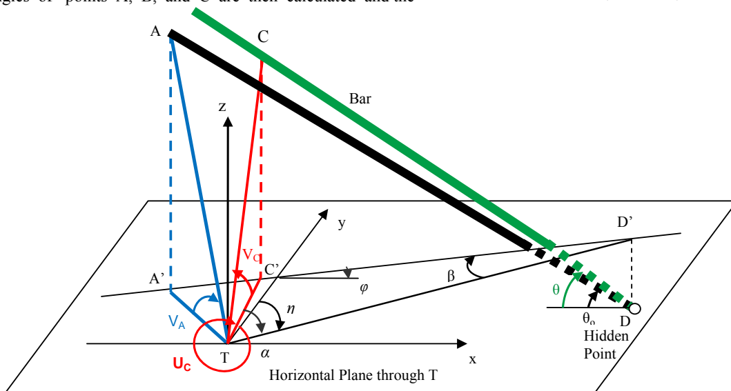
Fig. 2 Geometry of changing the bar vertical angle \theta
