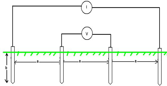
Fig. 2 Wenner Method for Soil Resistivity Test
