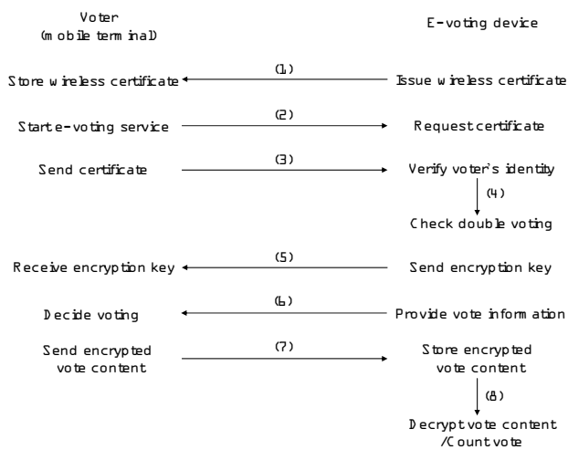
Fig. 2 E-voting process using a mobile terminal
