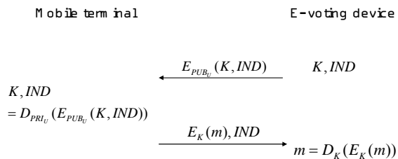
Fig. 4 Transferring secret key and vote content
