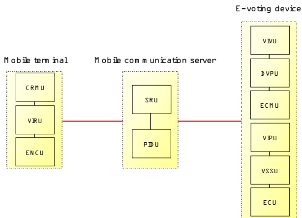
Fig. 1 E-voting system using mobile terminal
