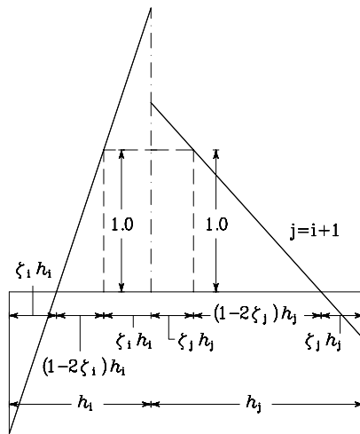
Fig. 2. Base functions w_i ; 2 \leq i \leq n-1 .
