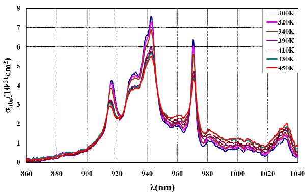
Fig. 4 Experimental measured absorption spectrum of 25at% Yb:YAG in the range of 300-450°K
