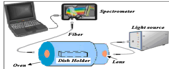
Fig. 2 Schematic view of the experimental setup for measuring the optical absorption of the disk crystal
