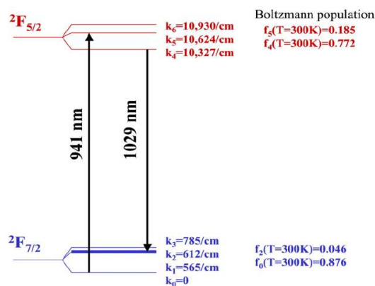
Fig. 1 Energy level scheme of Yb:YAG. f i 's are the relative thermal occupancies and the k i 's denote the wave number for different levels with regard to the ground level [6]
