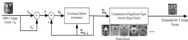
Fig. 4 Dimension reduction Block diagram
