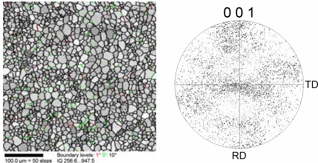
Fig. 1 Initial matrix and the corresponding \{100\} pole
