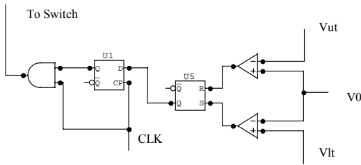
Fig 3 Control Logic
