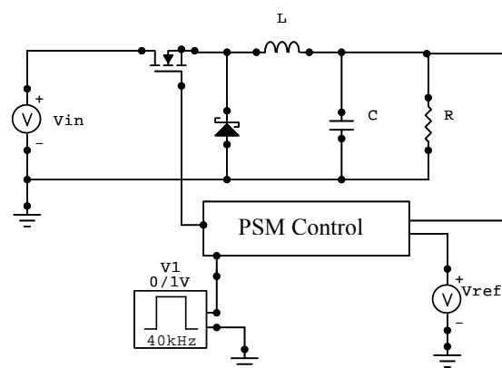
Fig. 1 Pulse Skipping Modulated Buck Converter
