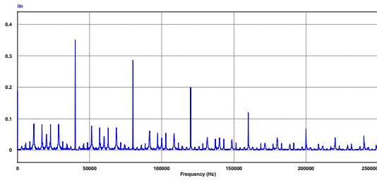
Fig. 7. Input Current Harmonic Spectrum - PSM Converter
