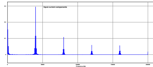
Fig. 6. Input Current Harmonic Spectrum - PWM Converter
