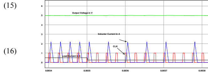
Fig. 5 Output voltage for step decrease in load current
