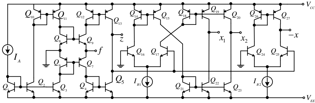
Fig. 3 Internal construction of MO-CFTA
