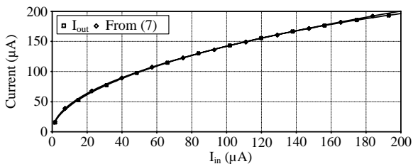
Fig. 4 DC transfer characteristic of the proposed circuit
