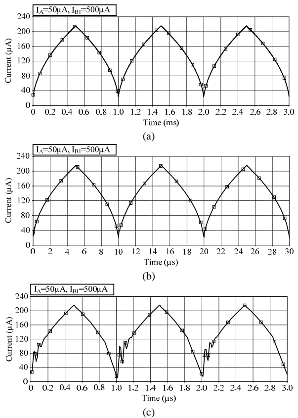
Fig. 5 The results of output current for different various input frequencies (a) 1kHz (b) 100kHz (c) 1MHz
