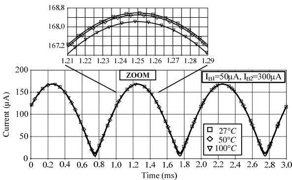
Fig. 8 The output deviations for different temperature values
