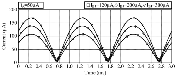
Fig. 7 The result of output current for different I_{B1}
