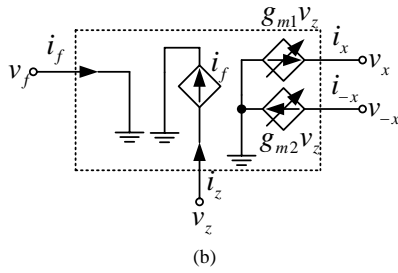
Fig. 1 MO-CFTA (a) schematic symbol, (b) equivalent circuit
