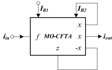
Fig. 2 Circuit diagram of current-mode square-rooter
