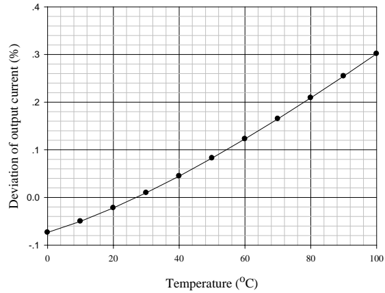
Fig. 9 The amplitude deviation of the output current for temperature variations
