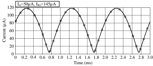
Fig. 6 The transient response of output current to a sinusoidal signal
