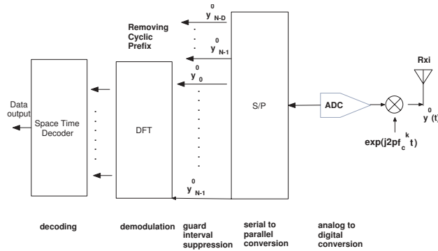
Fig. 3. Receiver architecture
