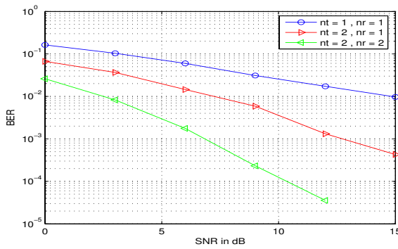
Fig. 7. BER plotted against SNR for orthogonal STBCs of selective-fading i.i.d. Rician channel with K = 3 and L = 4 .
