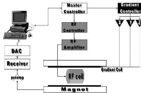
Fig. 2. MRI System from Instrumentation point of view [11]
