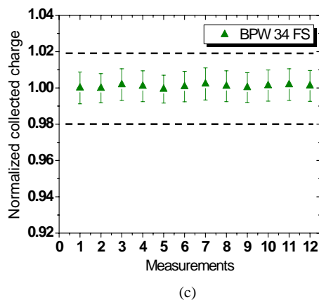
Fig. 7 Loss of sensitivity to 670 mGy accumulated air kerma of the three devices: (a) OP520 and (b) OP521 phototransistors; and (c) BPW34FS photodiode.
