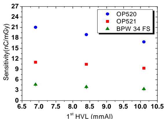
Fig. 5 Energetic dependence of the three devices: OP520 and OP521 fototransistors and BPW34FS photodiode
