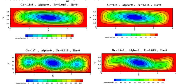
Fig. 3a Effect of Grashof number on streamlines
