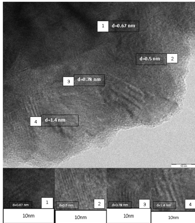
Fig. 9 TEM micrograph of "as milled" Cu-20% WC-5%Ti. Milled for 10 hours in closed air
