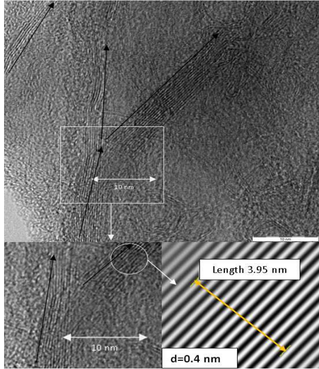
Fig. 8 TEM micrograph of "as received" titanium powder
