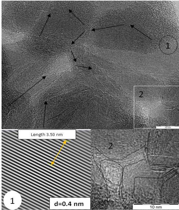
Fig. 6 TEM micrograph of "as received" Cu powder
