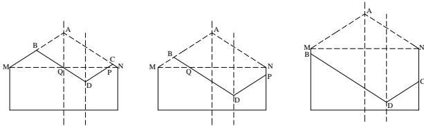
Fig. 8 Height of stored solids
