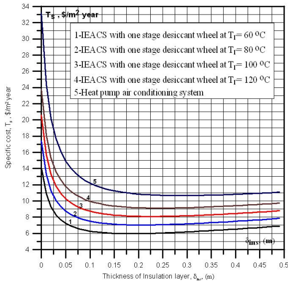
Fig. 14. Specific costs T_s , $/m 2 per year, for IEACS with one stage of desiccant wheel system for conditions of Egypt, city Aswan depending on the thickness \delta_{ins} , m of the building envelope.
