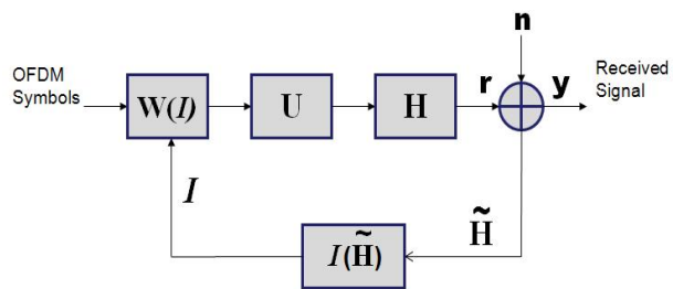
Fig. 2. Block Diagram of Feedback Model
