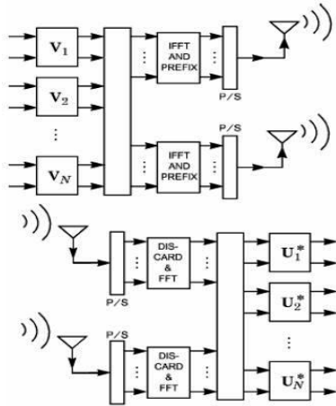
Fig. 3. SVD in MIMO-OFDM
