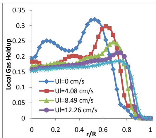
Fig. 6 (b) Radial distribution of Gas Holdup profiles for U_g=10.19 cm/s
