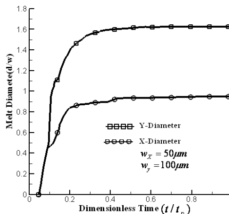
Fig. 13 Melting pool diameter on the x and y axes versus time for elliptical laser beam in continuous heat flux case
