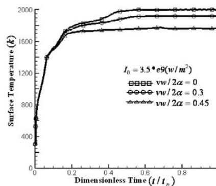
Fig. 7 Surface center point temperature with respect to the time at various speeds and intensity of I_0 = 3.5 \times 10^9 (W / m^2) in continuous heat flux case
