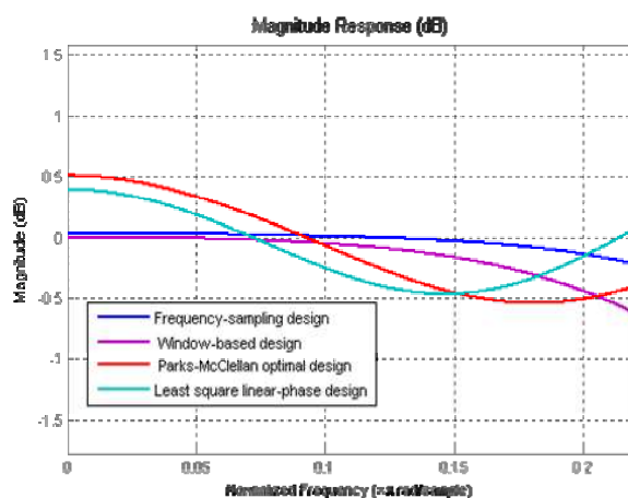
Fig. 3 Zoomed passband
