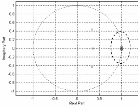
Fig. 8 Pole/zero plot
