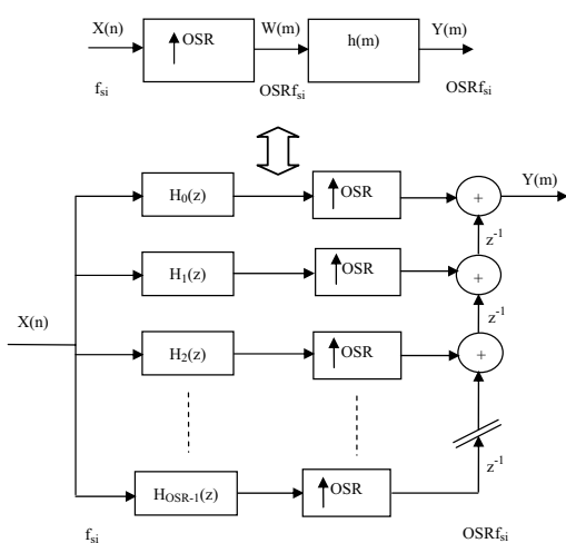
Fig. 4 Polyphase interpolation
