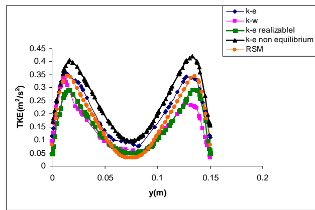
Fig. 7 Plot of kinetic energy between ribs 5 and 6
