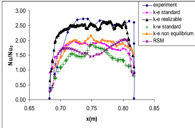
Fig. 4 Non dimensional Nu number between ribs 5 and 6
