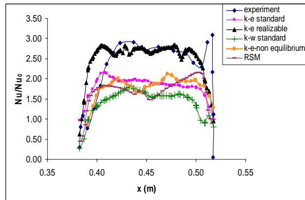
Fig. 3 Non dimensional Nu number between ribs 2 and 3
