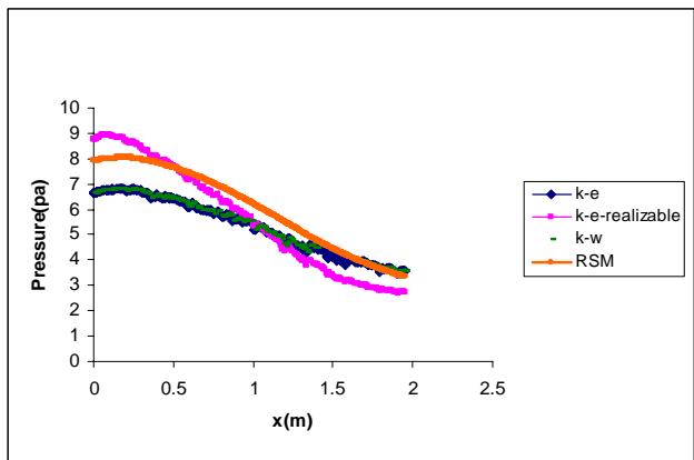
Fig. 5 Pressure drop along the channel
