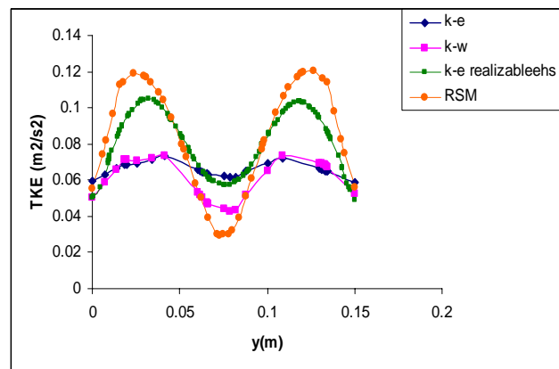
Fig. 8 Plot of kinetic energy after the last rib
