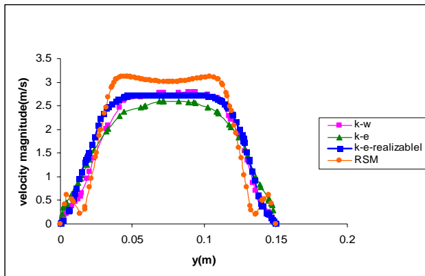
Fig. 9 Velocity profile between ribs 1 and 2
