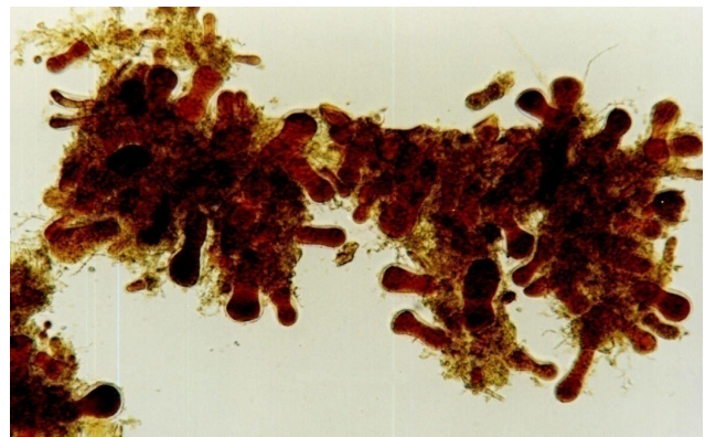
Fig. 2 Microscopic observation of pure anaerobic fungi in media (After three sub culture)
