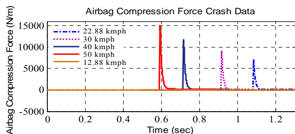
Fig. 14 Airbag compression force during various crashes
