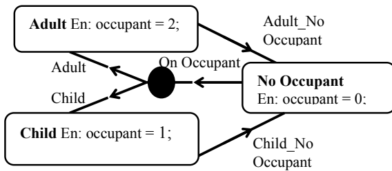
Fig. 3 Occupant sensing state flow controller
