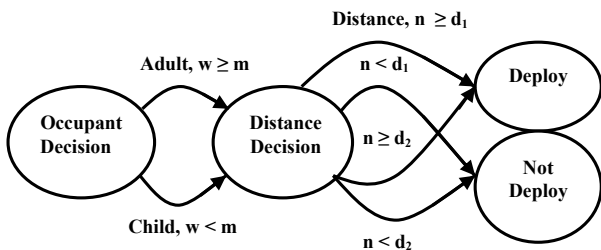
Fig. 6 State diagram of the safe distance decision
