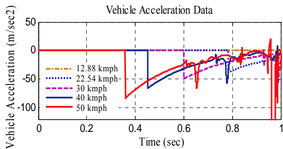
Fig. 13 Vehicle acceleration Crash data at various speeds
