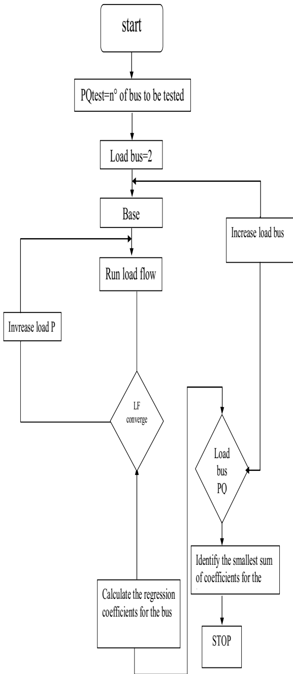
Fig. 3 Flow chart computation latest bus
