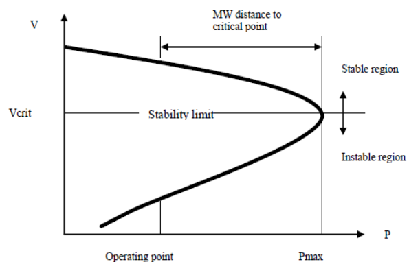
Fig. 1 PV curve
