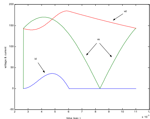
Fig. 6 MATLAB simulation of the single-phase diode bridge rectifier using analytical model
