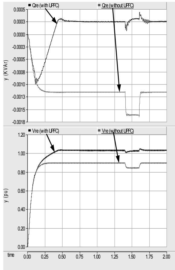
Fig. 9 Fuzzy controller results at fault condition
