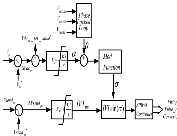
Fig. 2 PI controller based control mechanism
