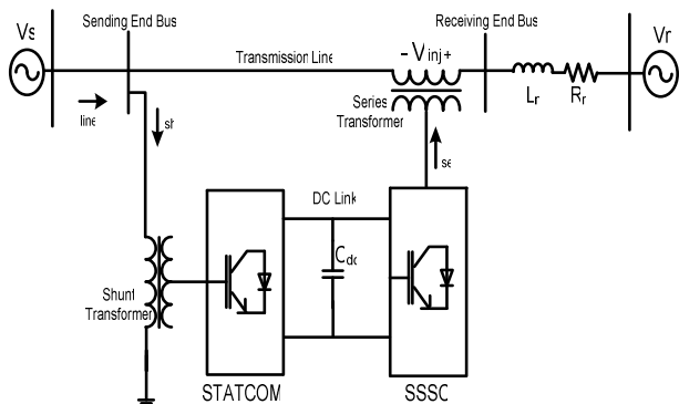
Fig. 1 Basic scheme of UPFC system
