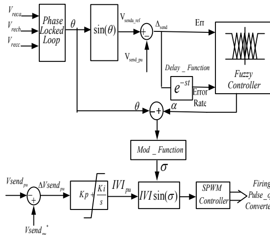
Fig. 3 Fuzzy controller based control mechanism
