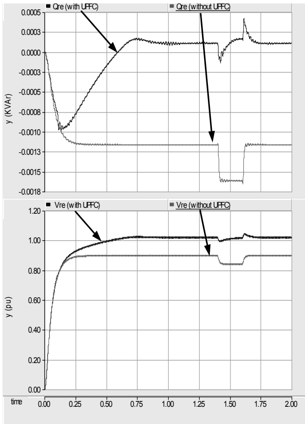
Fig. 8 PI controller results at fault condition
