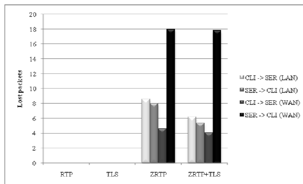
Fig. 12 \mu -law codec Packet Lost
