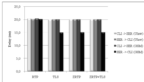
Fig. 7 Delay WAN Scenario
