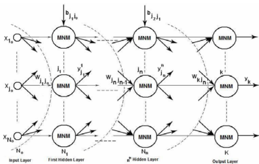
Fig. 3 Pi neuron based ANN
