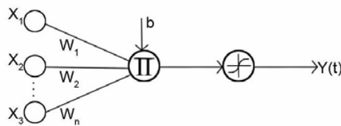
Fig. 2 A single multiplicative neuron
