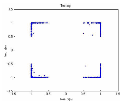
Fig. 5 (b) 4 QAM signal output of pi network
