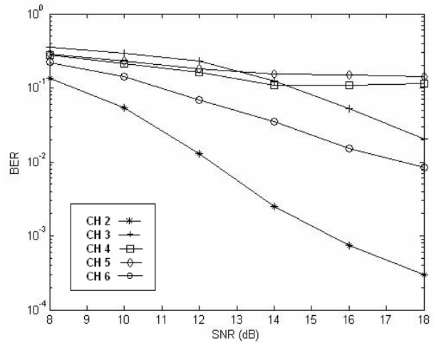
Fig. 4 BER for various channels
