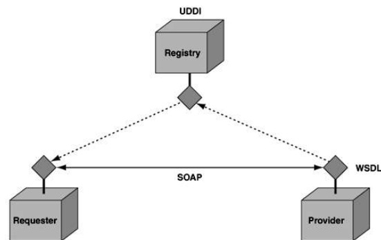
Fig. 1 Basic Web service architecture
