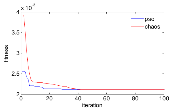
Fig. 6 Convergence of PSO and chaos algorithms
