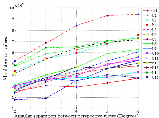
Fig. 10 Absolute pixel error for 15 bags at 2°, 3°, 4°, 5° and 6° of separation
