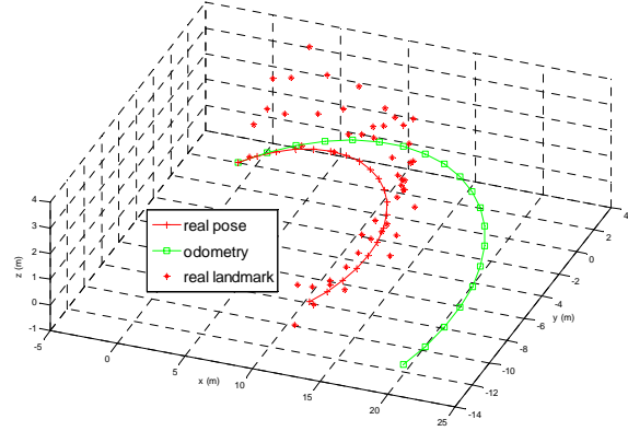
Fig.8. simulation environment
