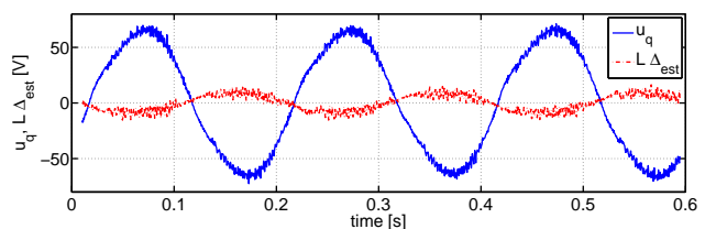
Fig. 4. Voltages u_q and L\Delta_{est}
