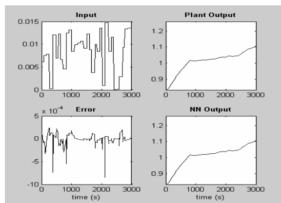
(a) Training (input-output) data; ANN error and output
