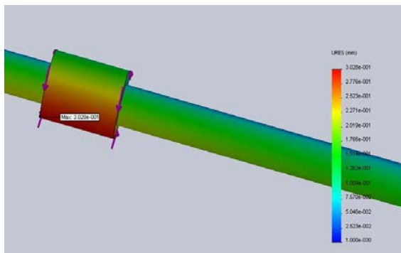
Fig. 7 Deflection of the Front Shaft
