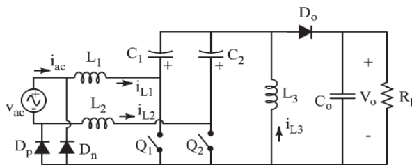
Fig. 4 Bridgeless DCM SEPIC AC-DC converter [10]
