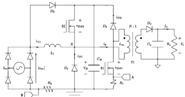
Fig. 2 SS PFC with boost and clamped flyback converters [6]
