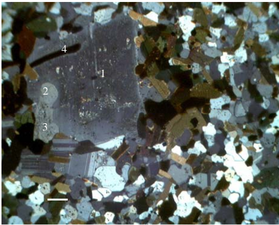
Fig. 9: Photomicrograph of Hybrid rock (H2 b) showing plagioclase xenocryst (1), inherited quartz (2), inherited feldspar (3) and biotite intergrowth (4). Bar Scale is 1 \mu m.
