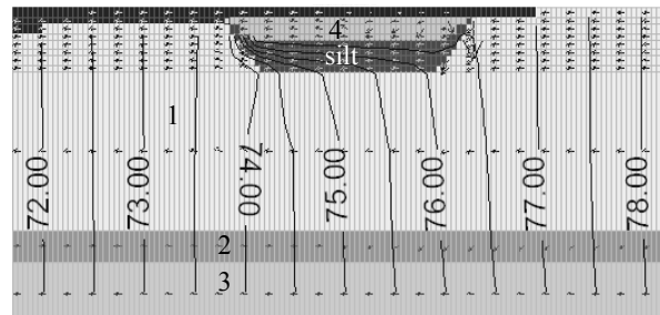
Fig. 8: Numerical modeling of the water table deformations in a quarry lake in presence of silt deposition both on the bottom and along the scarps for excavation depth very less than the first aquifer thickness
