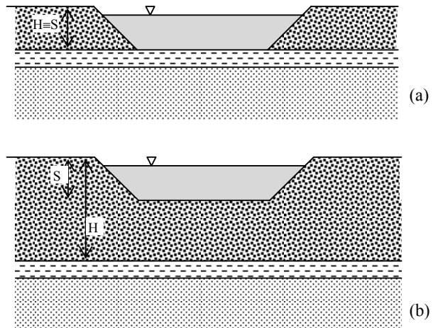
Fig. 3: Hydrogeological scheme used for modeling: (a) the excavation depth S is equal to the thickness of the first aquifer H; (b) S is lower than H
