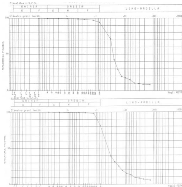
Fig. 1: Grain size distributions of the fine wastes of a quarry. (a): 11% of sand, 80% of silt, 8% of clay; (b): 29% of sand, 64% of silt, 7% of clay
