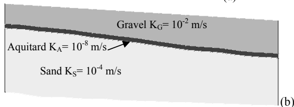
Fig. 13: (a) Modeling domain with the hydraulic conductivity distribution of the first layer and the model boundary conditions: constant head along the border domain, constant flow with squares and flow dependent head with circles (N1, N2 and N3 are the springs for which the modeling results will be shown in the following); (b) N-S section of the domain
