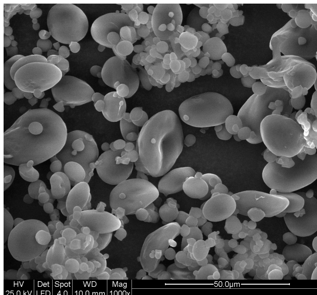
Fig. 1 Starch recovered inside dialysis tubing without α-amylase
