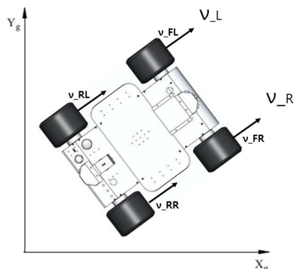
Fig. 1 Wheel velocities
