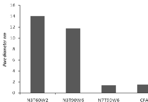
Fig. 7 Pore diameter original and treated CFA N3T60W2 means NaOH concentration of 3M, Temperature of 60°C, reaction time of 2 hours
